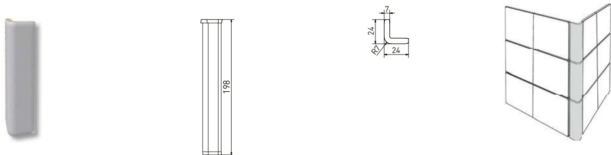
colț exterior duș / outside edge - shower piece | GSEAP... | GSEAPF... | 198×24×7 mm
